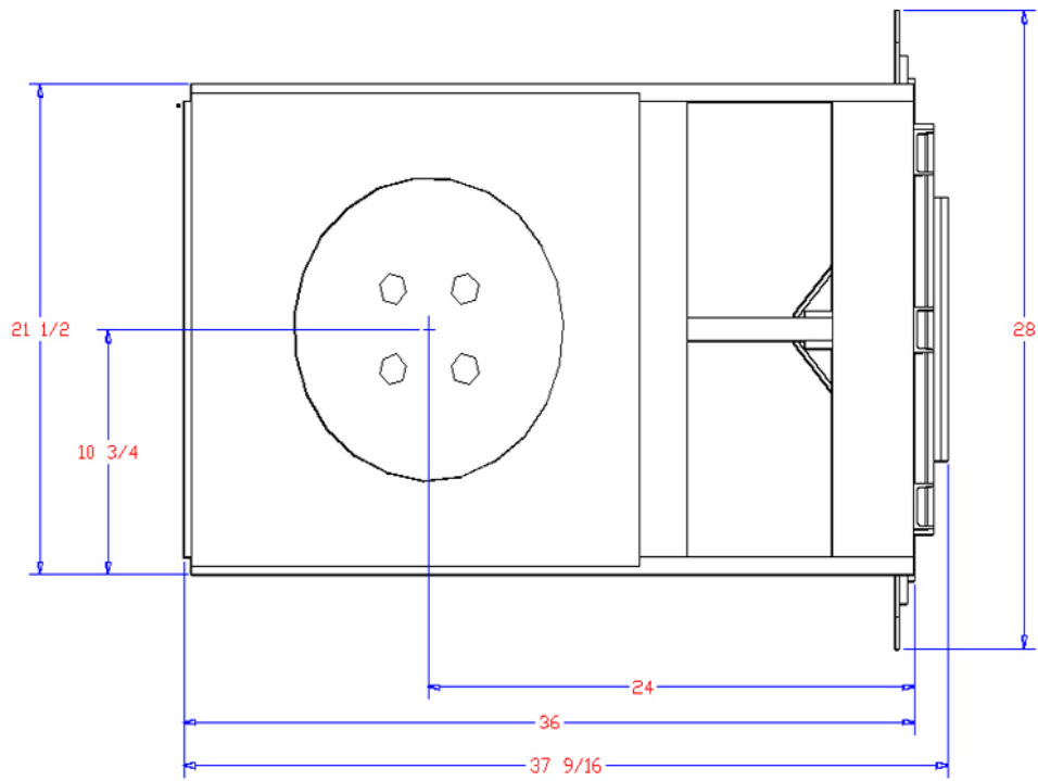
Liftomatic L4C Forklift Carrier Mounted Drum Handler
